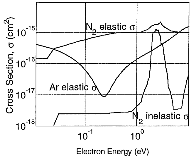
Figure 6. Electron interaction cross sections for argon and nitrogen.
