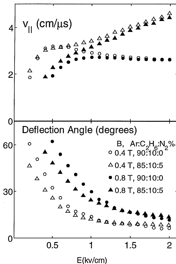
Figure 11. Deflection angles are reduced by \text{N}_2 additions for an \text{Ar}:\text{C}_2\text{H}_6 mixture.
