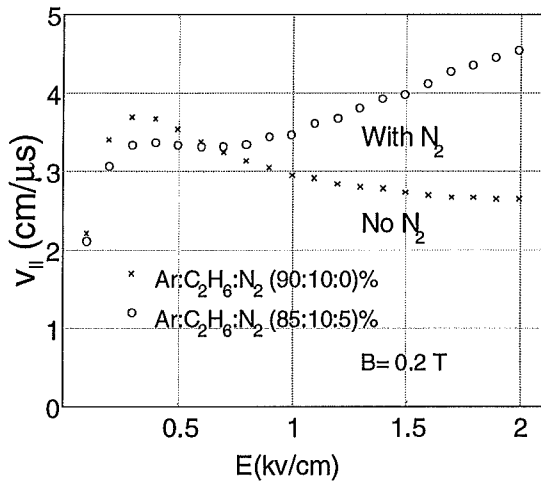
Figure 7. Effect of small N_2 additions on drift velocity.
