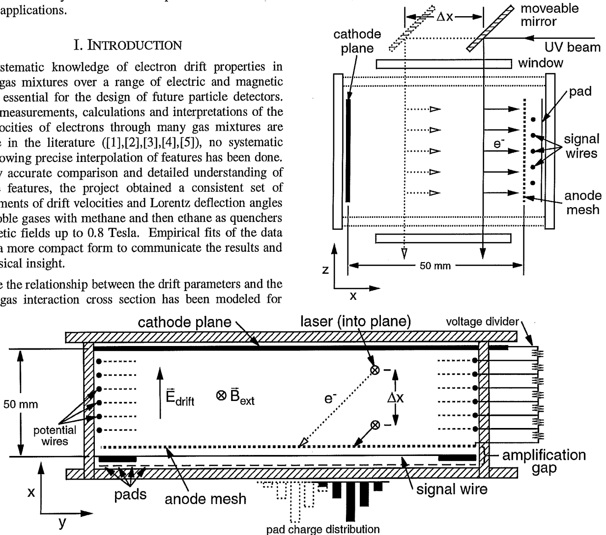
Figure 1. Chamber diagram, xz projection (top) and xy projection (bottom).
