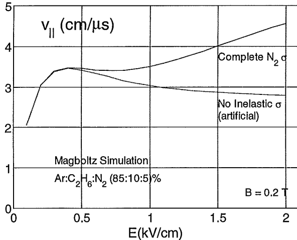
Figure 8. Simulations confirm the effect of N_2 's inelastic component.
