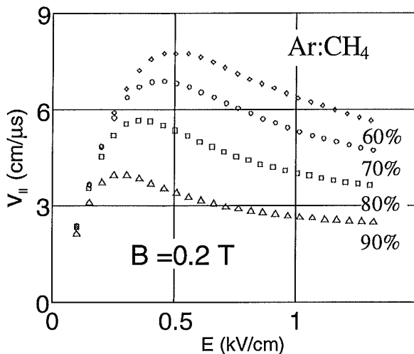
Figure 2. Argon-based mixtures with varied percentages of methane quencher.
